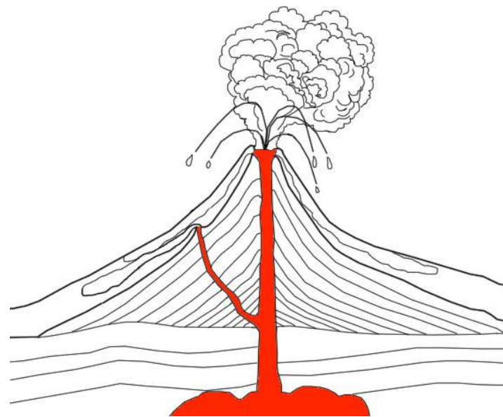
magma
