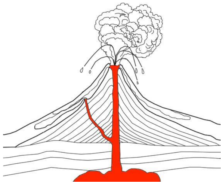
magma
