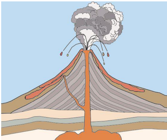
volcan
